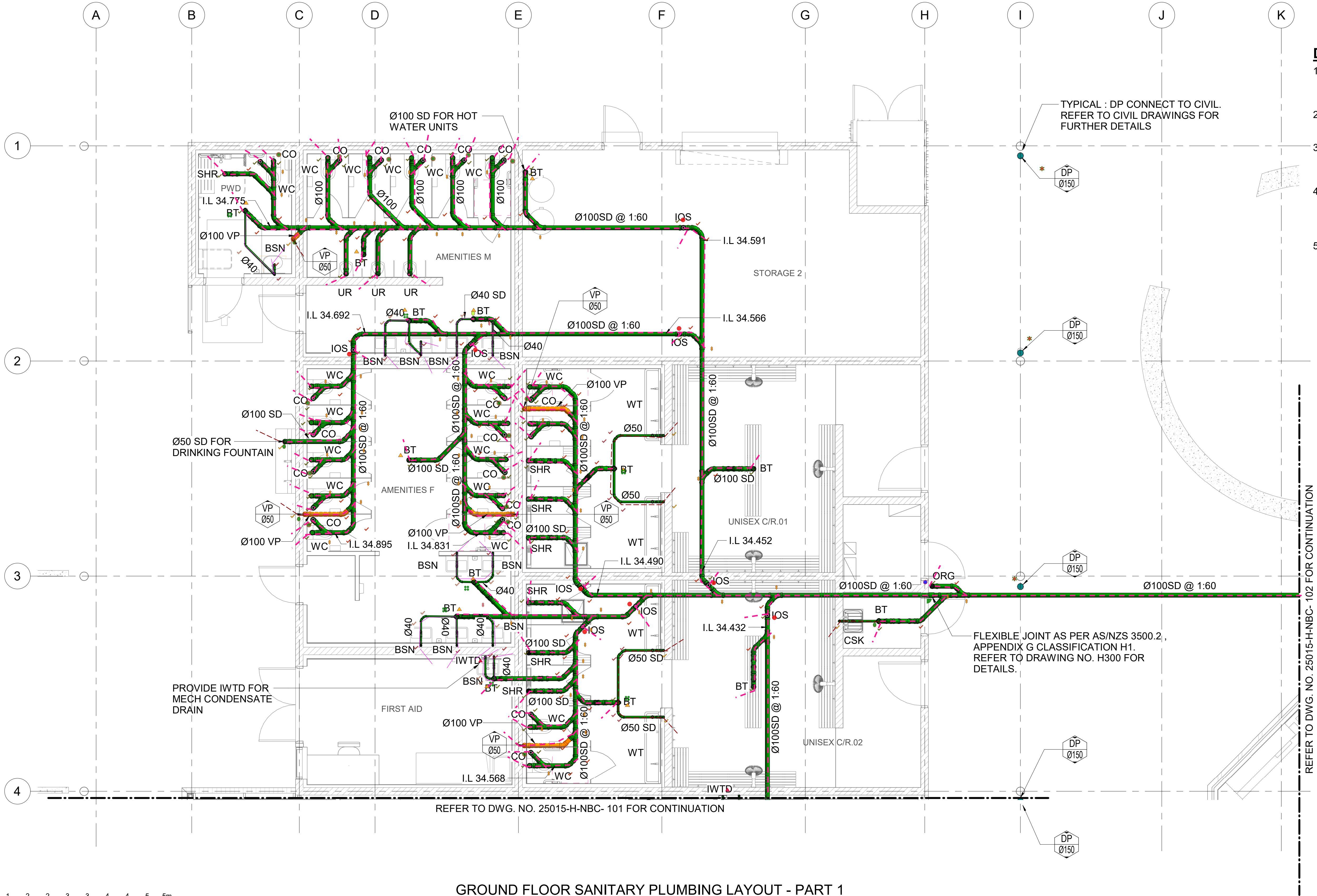
GROUND FLOOR SANITARY PLUMBING LAYOUT - PART 1
